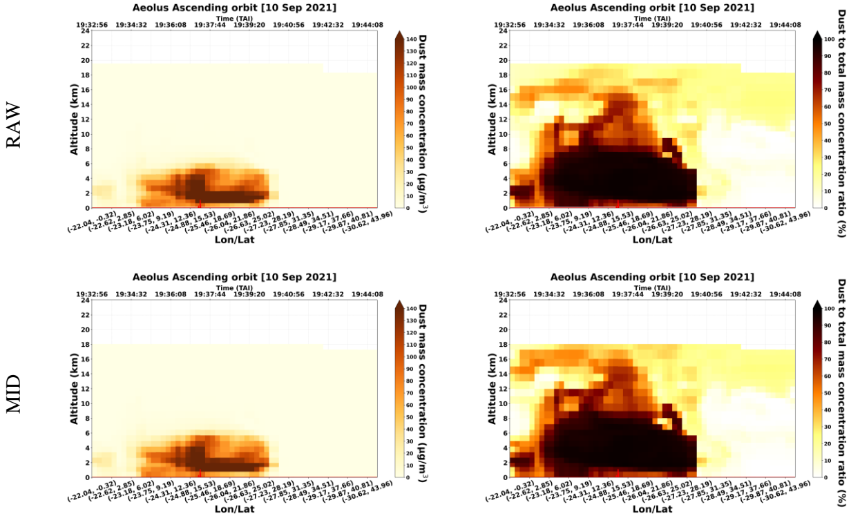
Figure 5.3: Vertical profiles of CAMS dust mass concentration and dust-to-total aerosol mass concentration ratio along the Aeolus orbit (id: 017679) provided in the regular (a, b) and middle-bin (c, d) vertical scales on the 10th of September 2021.
