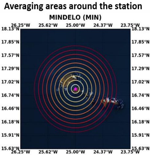
Figure 3.3: Averaging areas around the ESA-ASKOS domain.
